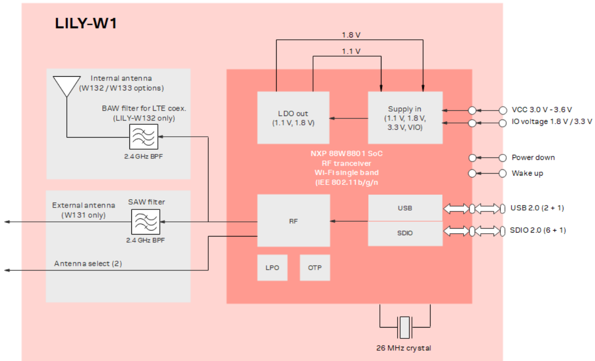
Figure 1: Block diagram of LILY-W1
