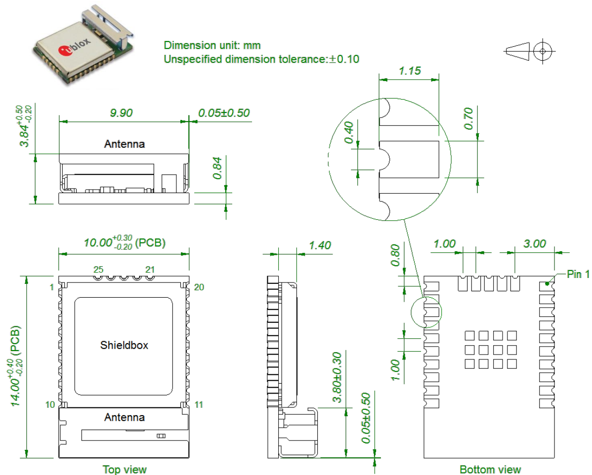
Figure 5: LILY-W132 and LILY-W133 dimensions
