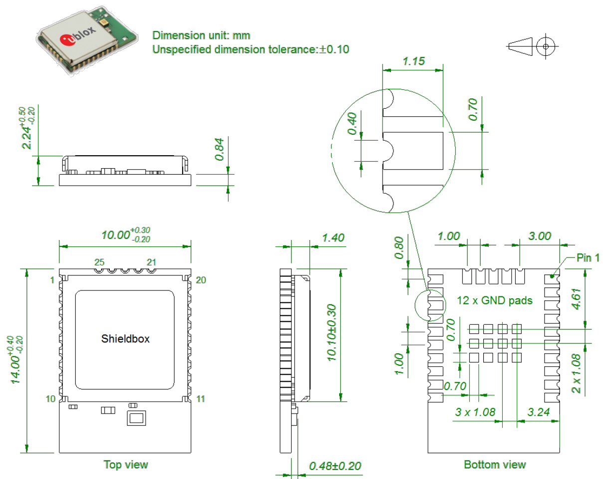
Figure 4: LILY-W131 dimensions
