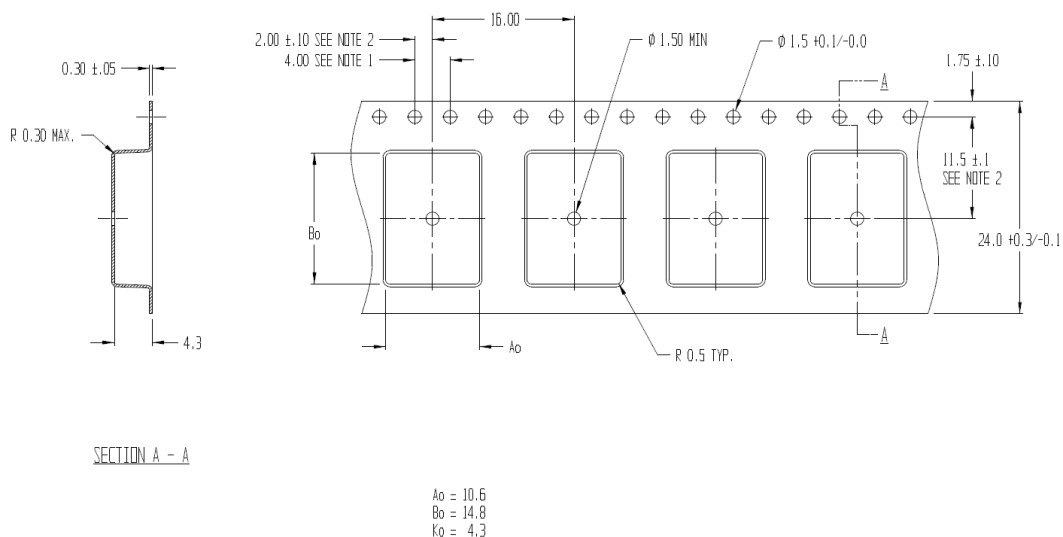
Figure 7: Orientation of LILY-W132 modules on tape
