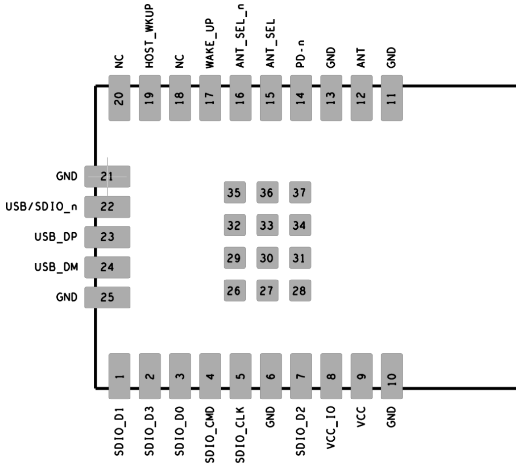
Figure 3: LILY-W1 series pin assignment (top view)
